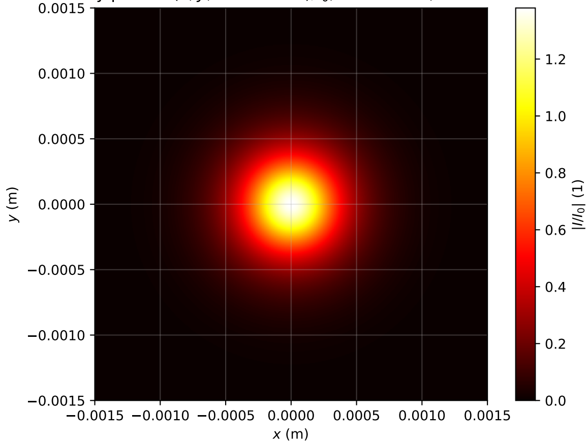
Intensity profile I(x, y, z = 0.955m)/I_0 , \text{Pin}=0.9\text{Pcr} , artificial time
